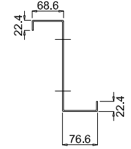
1 - 1 (t=3,0 mm)
