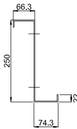
1 - 1 (t=2,0 mm)
