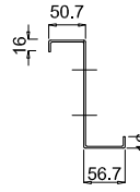
1 - 1 (t=2,0 mm)
