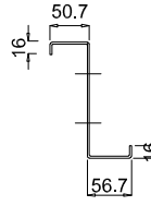
1 - 1 (t=2,0 mm)
