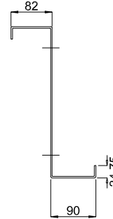
1 - 1 (t=2,0 mm)
