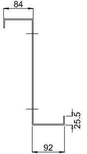
1 - 1 (t=3,0 mm)
