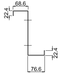
1 - 1 (t=3,0 mm)
