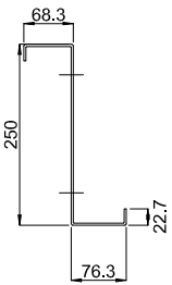
1 - 1 (t=3,0 mm)
