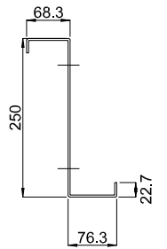
1 - 1 (t=3,0 mm)
