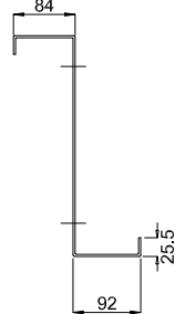
1 - 1 (t=3,0 mm)
