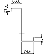
1 - 1 (t=2,0 mm)
