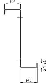
1 - 1 (t=2,0 mm)
