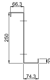
1 - 1 (t=2,0 mm)
