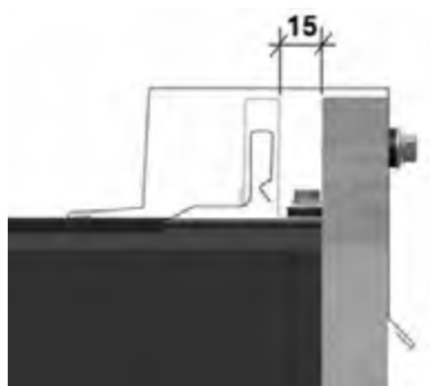
Figure 13. Distance between the sheet and the roof edge
