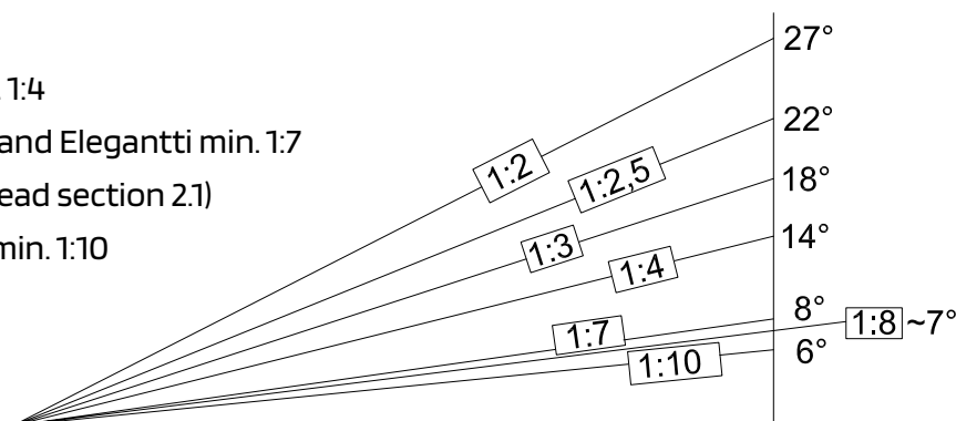
Figure 4c. Minimum slopes for various roofing types
