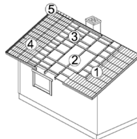
Figure 55. Renovation of an old seam metal roof
