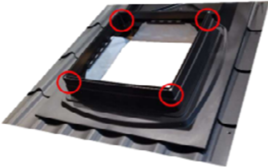
Figure 47. Screw placement
