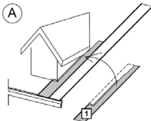
Figure 23 A. Cutting the sheet [1] at the eaves
