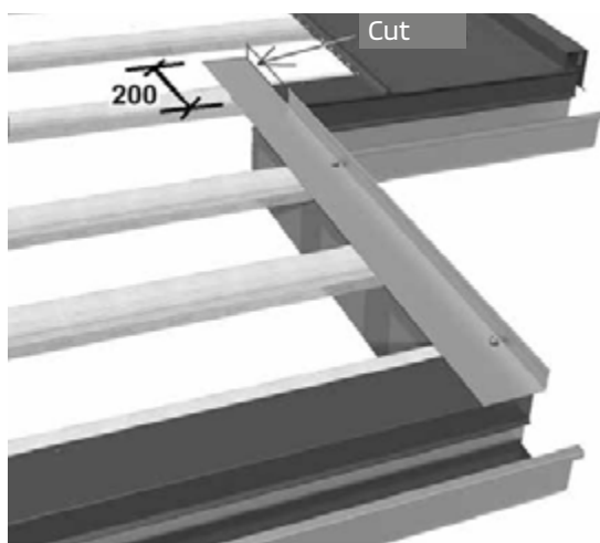
Figure 26. Lower eaves flashing
