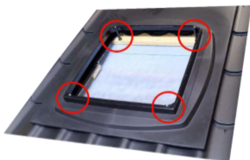
Figure 45. Fixing the base to the battens with screws through the support sleeves
