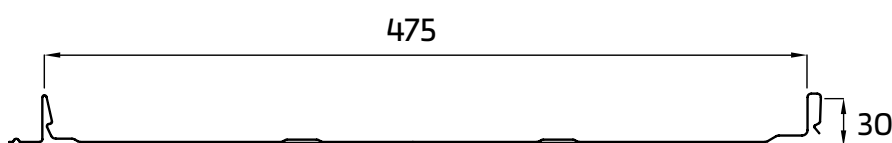
Figure 4b. PROGANTTIJ nominal cross-section dimensions in accordance with the tolerances specified in SFS EN-508-1
