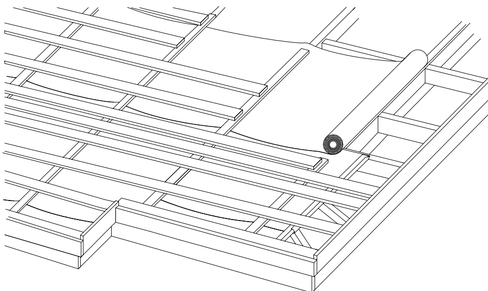
Figure 7. Underlay structure
