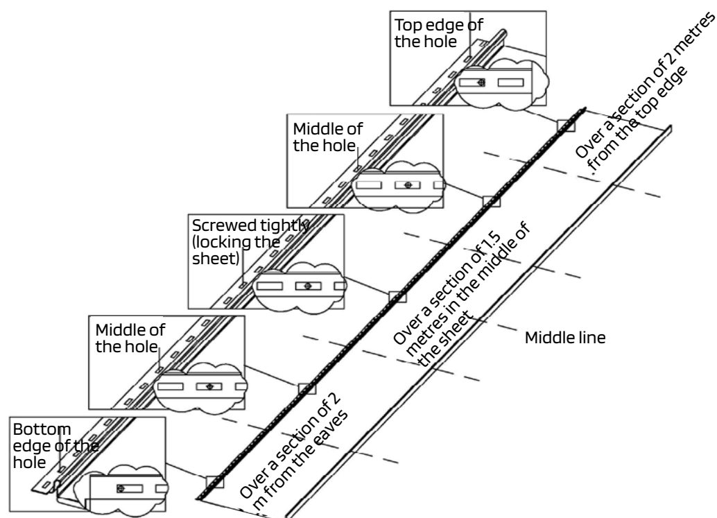
Figure 14. Placement of the 4.2 x 25 stainless steel screws in the various parts of the roofing sheet
