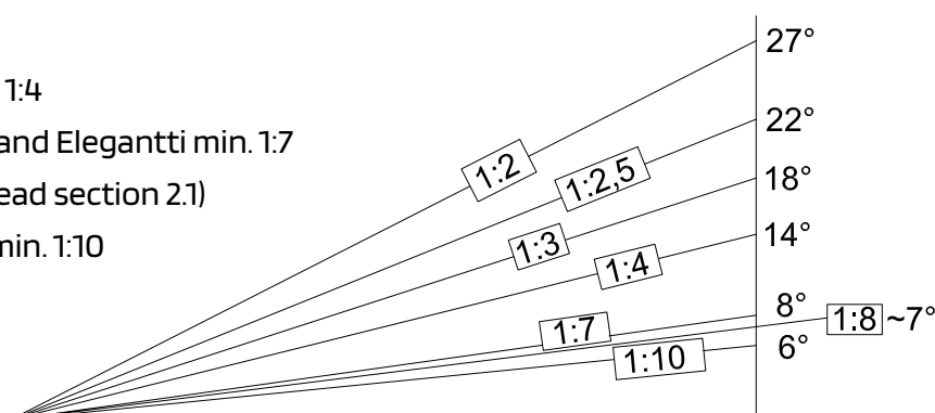
Figure 4c. Minimum slopes for various roofing types
