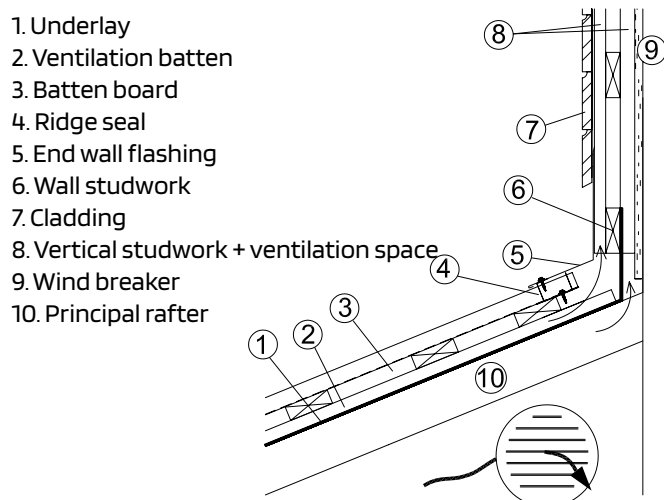
Figure 33. Crosswise roof-to-wall junction
