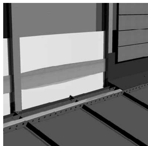
Figure 34. Crosswise roof-to-wall junction
