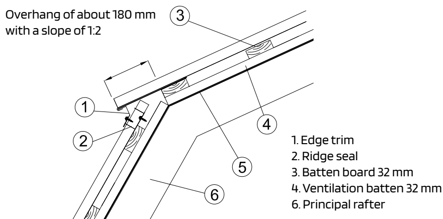
Figure 36. Gambrel roof edge
