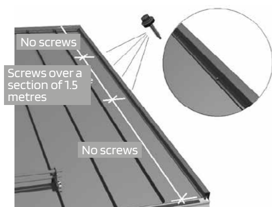
Figure 24a. Attaching the gable flashing to the batten
