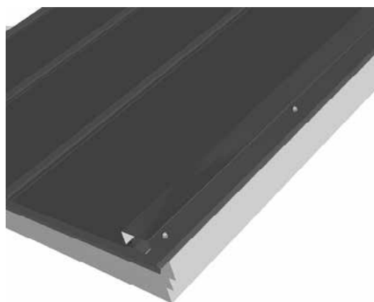
Figure 24b. Attaching the gable flashing to the fascia
