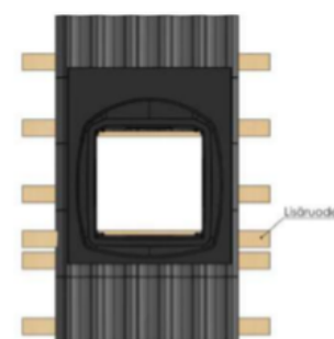
Figure 41. Add extra batten if necessary
