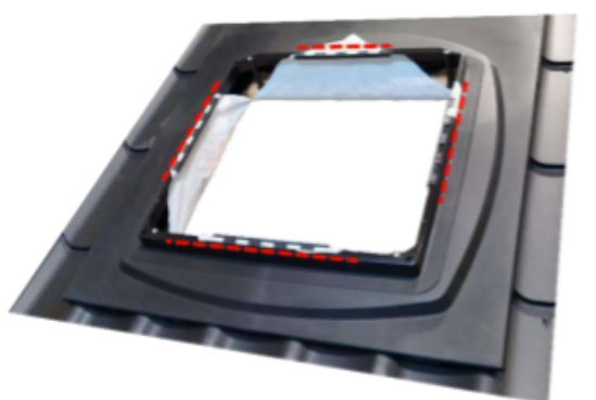
Figure 46. Underlay cut and fixed to the base
